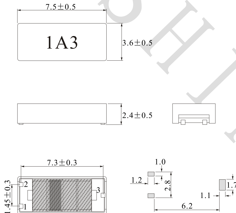
Pad layout
